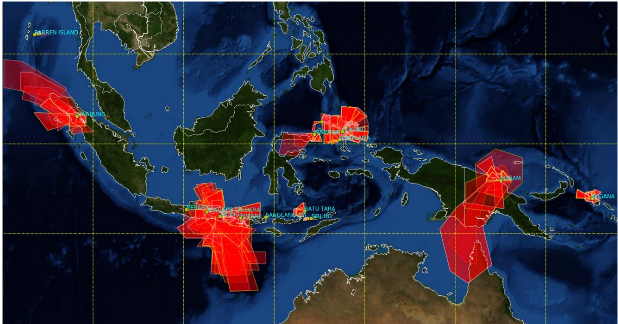
Figure 2 – Areas covered by volcanic ash forecasts during 2015
