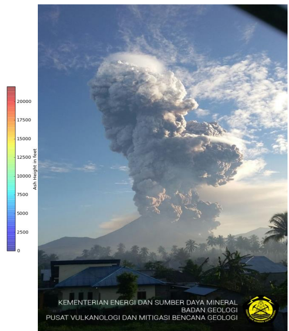
Figure 8: Soputan, 05 Jan 2016 2
